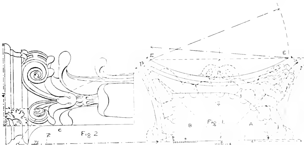
No. 102.—TO SET OUT CORINTHIAN COLUMN AND PLASTER CAPITALS.
